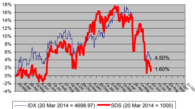
SDS v.s IDX Performance (20 Mar '14 - 30 Jun '15)
