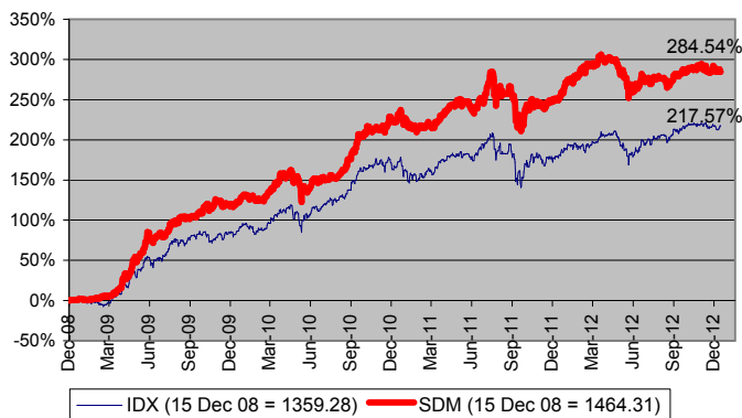
SDM v.s IDX Performance (15 Dec 08 - 28 Dec '12)
