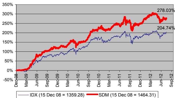
SDM v.s IDX Performance (15 Dec 08 - 31 Jul '12)
