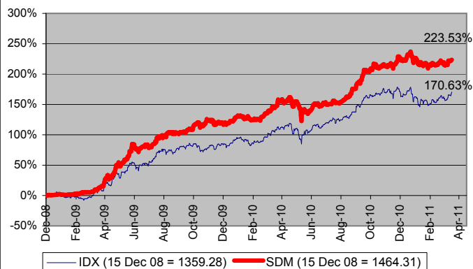
SDM v.s IDX Performance (15 Dec 08 - 31 Mar '11)
